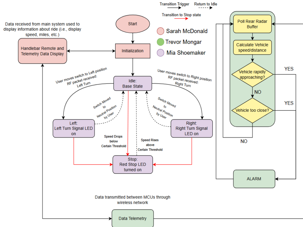
Figure 4.3 System Software Design by Authors
